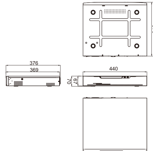
Figure 2-1 Dimensions (Unit:mm)
