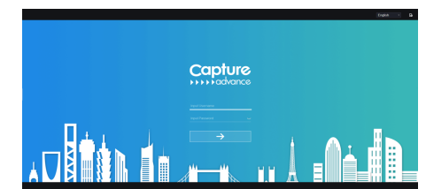
Figure 7-1 Login
